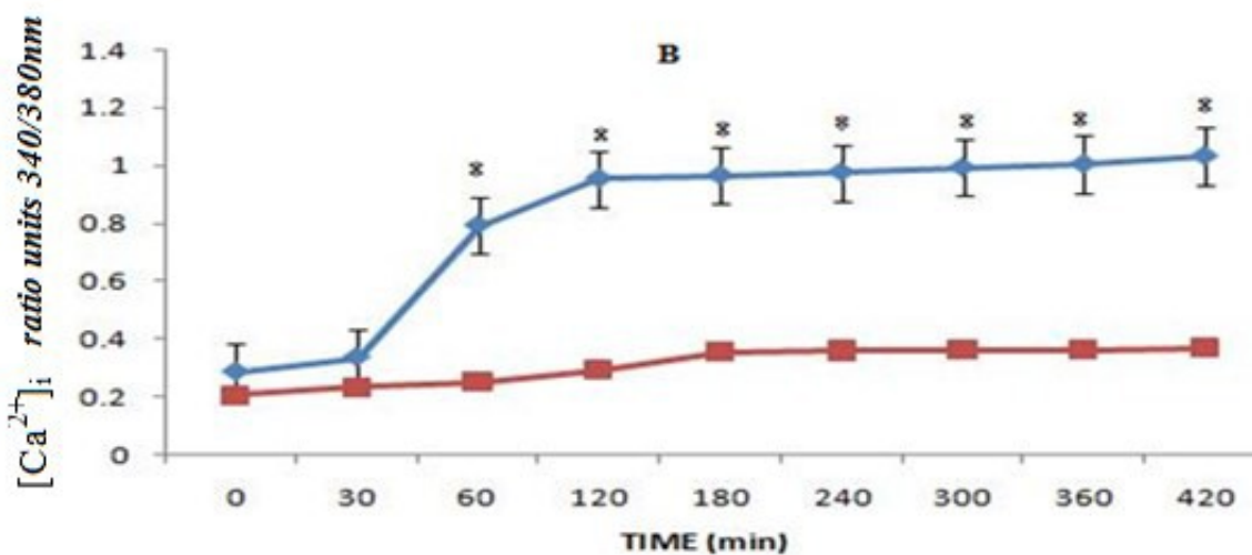
Figure 2. Time-course changes in [Ca^{2+}]_i expressed as fluorescence ratio units (intensity) in Fura-2 AM loaded U87-MG cell lines.
