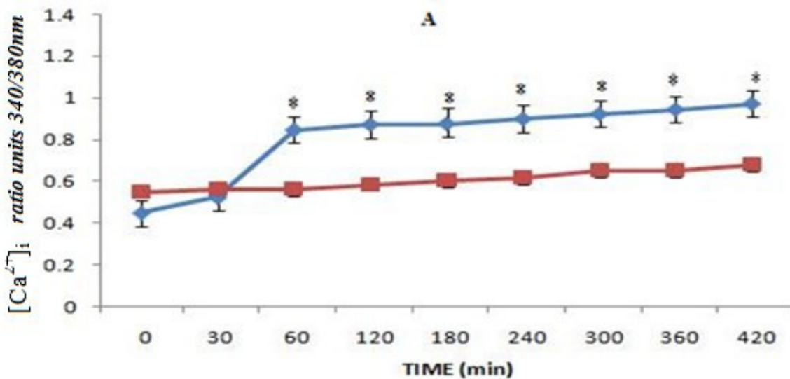
Figure 1. Time-course changes in [Ca^{2+}]_i expressed as fluorescence ratio units (intensity) in Fura-2 AM loaded 1321N1 cell lines
