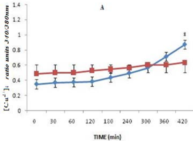
Figure 3. Time-course changes in [Ca^{2+}]_i expressed as fluorescence ratio units (intensity) in Fura-2 AM load-ed U87-MG cell lines.
